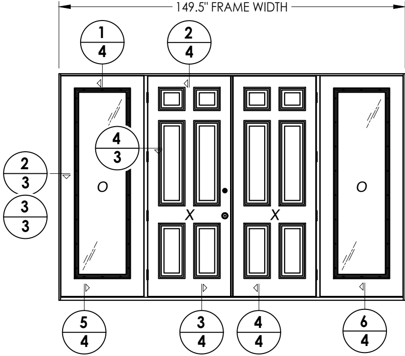
DOUBLE DOOR w/ SIDELITES (Shown with opaque door)
