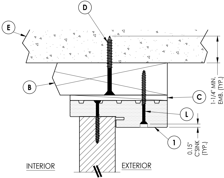
1 4 VERTICAL CROSS SECTION 2X Buck Construction - Sidelite Inswing Shown (Outswing Similiar)
