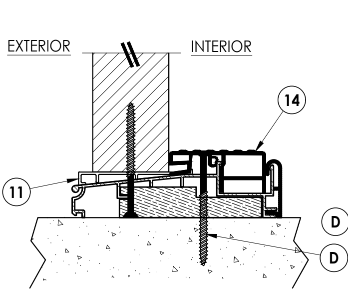
5 4 VERTICAL CROSS SECTION Outswing
