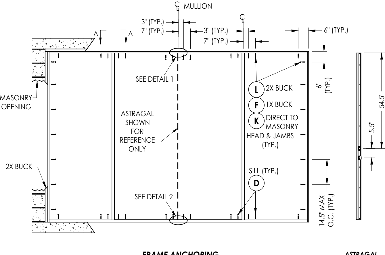
FRAME ANCHORING Masonry construction
