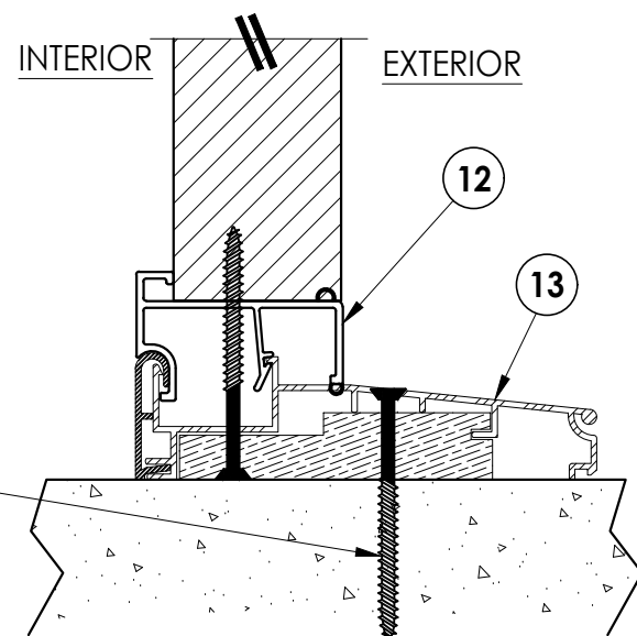
6 4 VERTICAL CROSS SECTION Inswing
