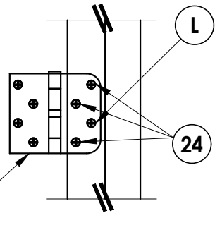
HINGE DETAIL
