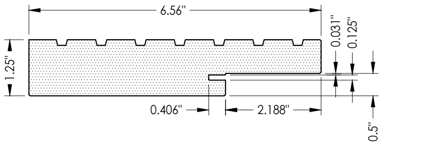
1 HEAD & SIDE JAMB 4Ever Frame (6-9/16")
