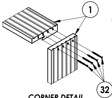
CORNER DETAIL @ HEAD (TYP.)
