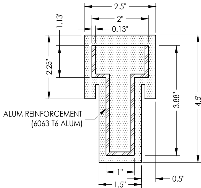
3 MULLION w/ ALUM REINFORCEMENT 4Ever Frame
