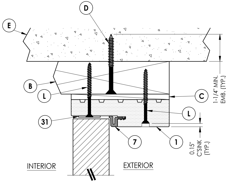
2 4 VERTICAL CROSS SECTION 2X Buck Construction - Door Inswing Shown (Outswing Similiar)
