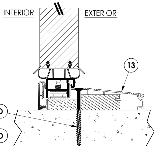
4 4 VERTICAL CROSS SECTION Inswing
