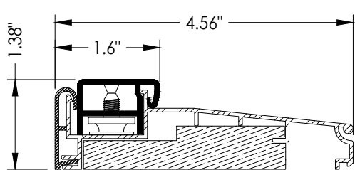
13 INSWING THRESHOLD WORLDWIDE
