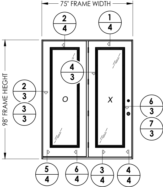
SINGLE DOOR (CENTER HINGED) w/ SIDELITE (Shown with glazed door)
